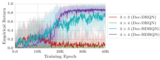
(a) Empirical returns during training. For batch of 50 randomly-initialized games.
